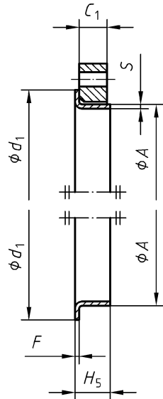
g) Type 02 and 37
