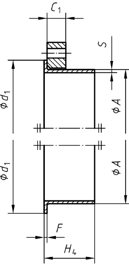
f) Type 02 and 36
