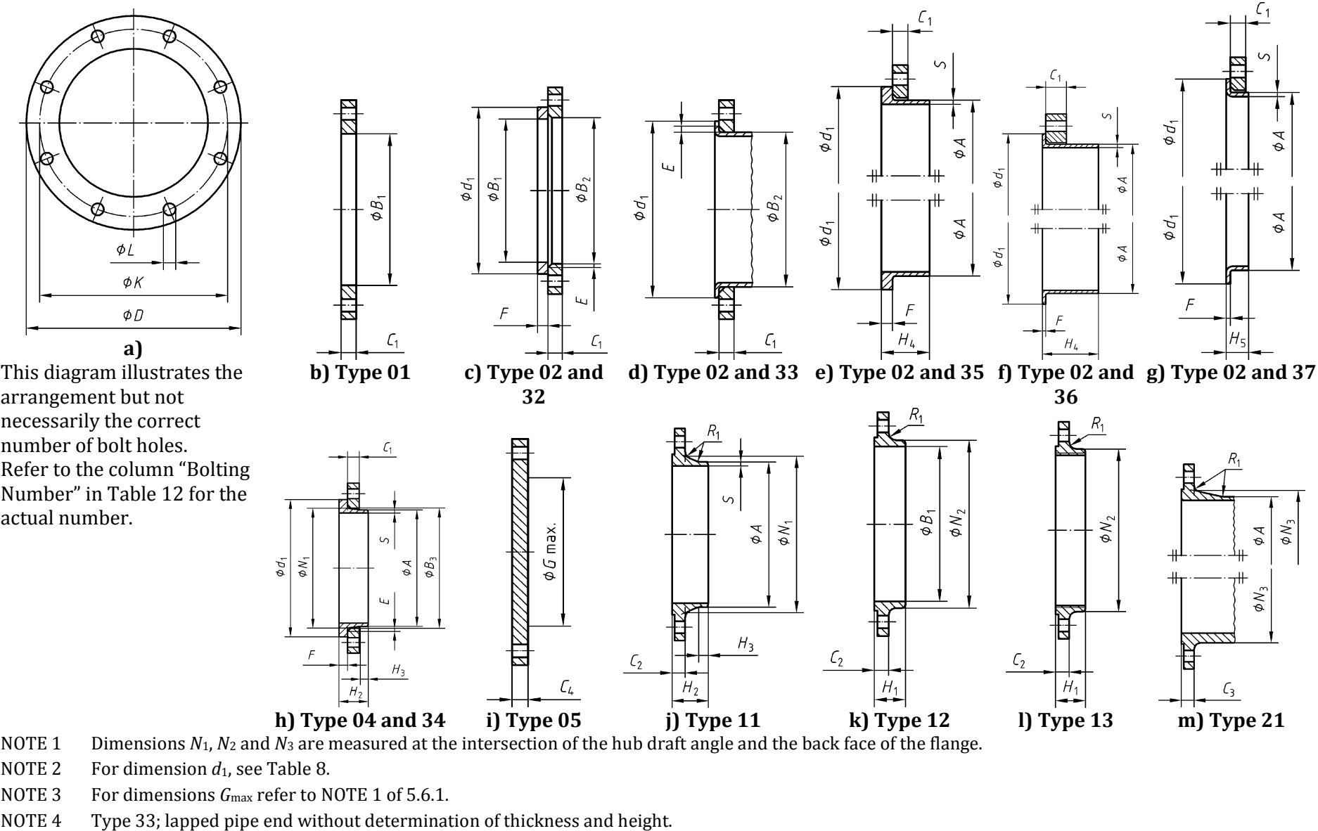
Figure 7 — Dimensions of PN 10 flanges
