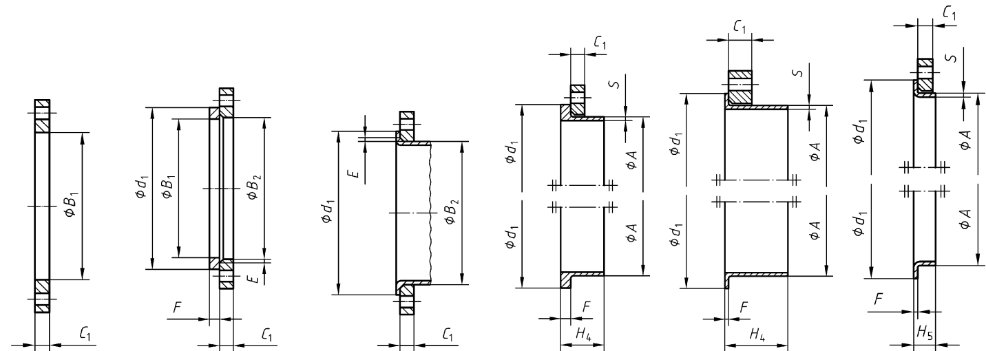
b) Type 01 c) Type 02 and 32 d) Type 02 and 33 e) Type 02 and 35 f) Type 02 and 36 g) Type 02 and 37
